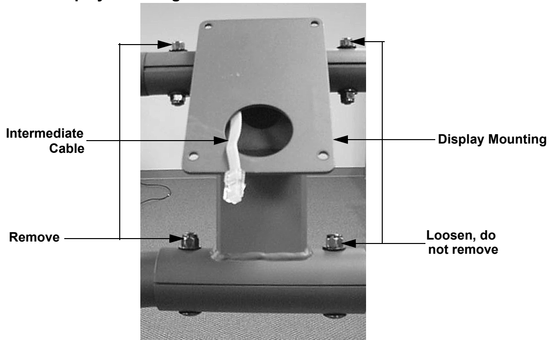
Diagram 7.5 - Display Mounting
