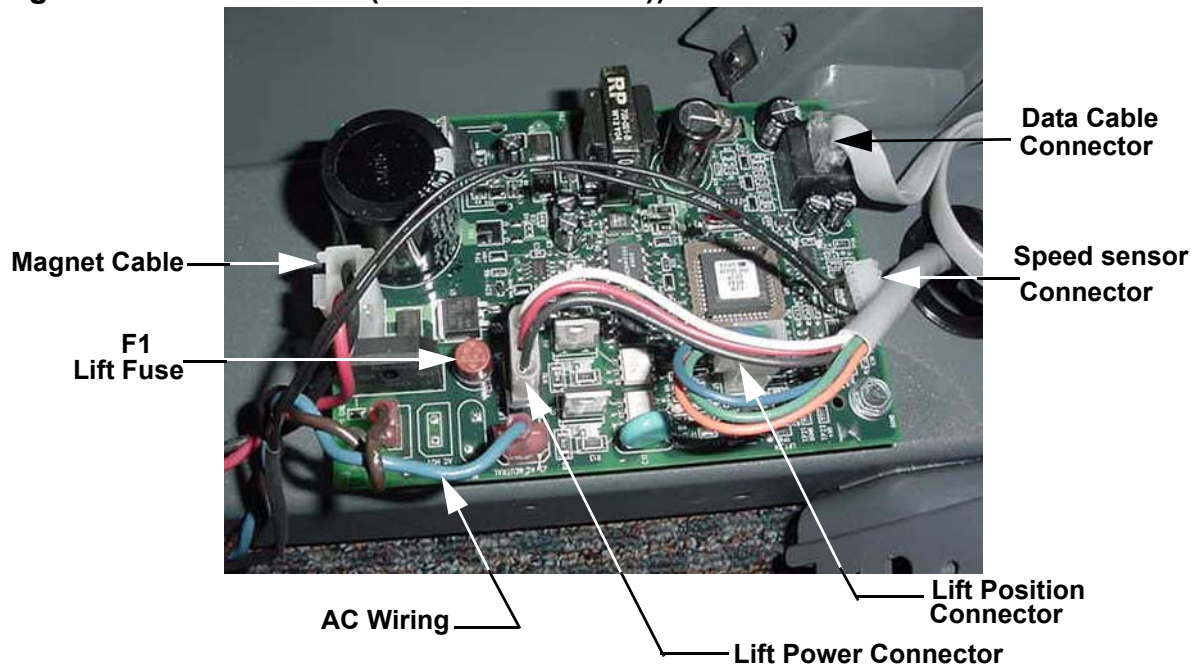
Diagram 7.4 - Lower PCA (serial code AMPF))
