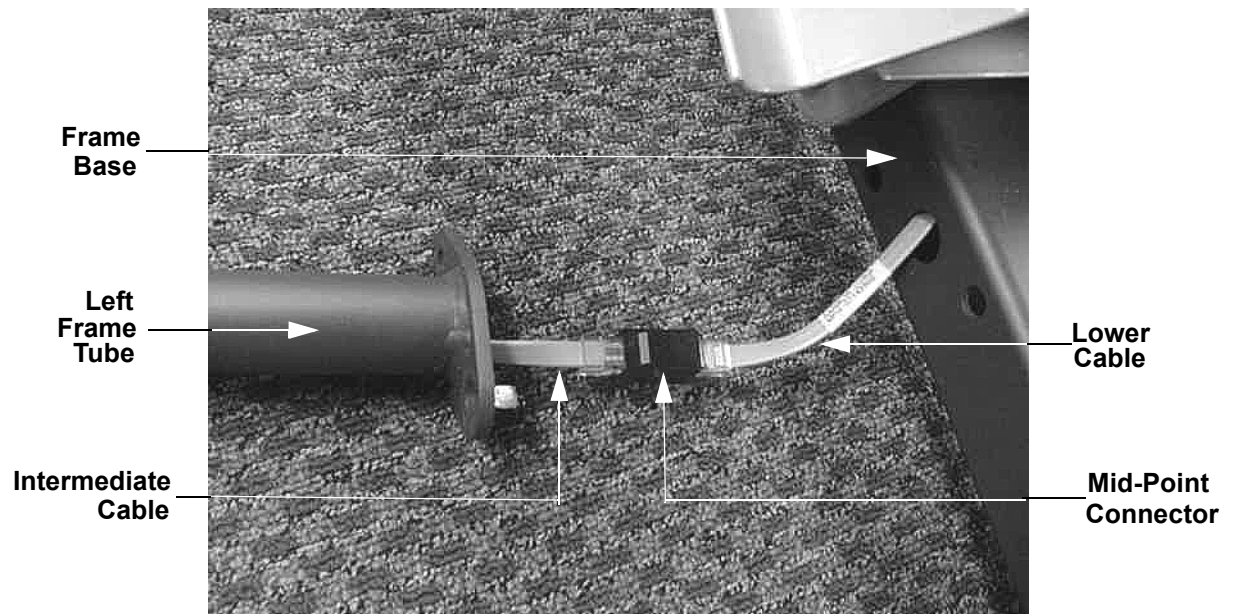
Diagram 7.6 - Interconnect Cables.
