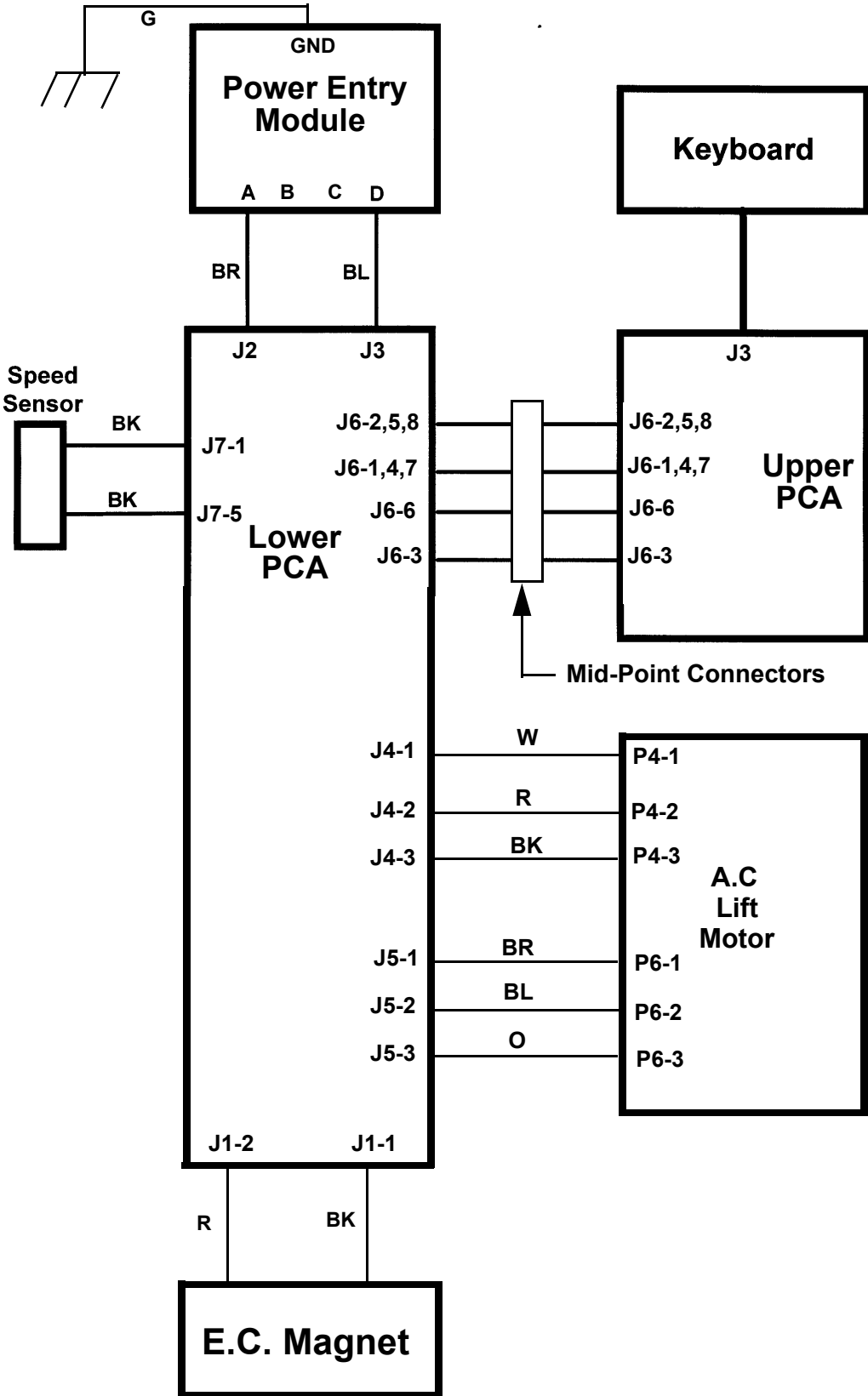
Wiring Diagram 8.3 - 5.17i (Serial code AMPF)
