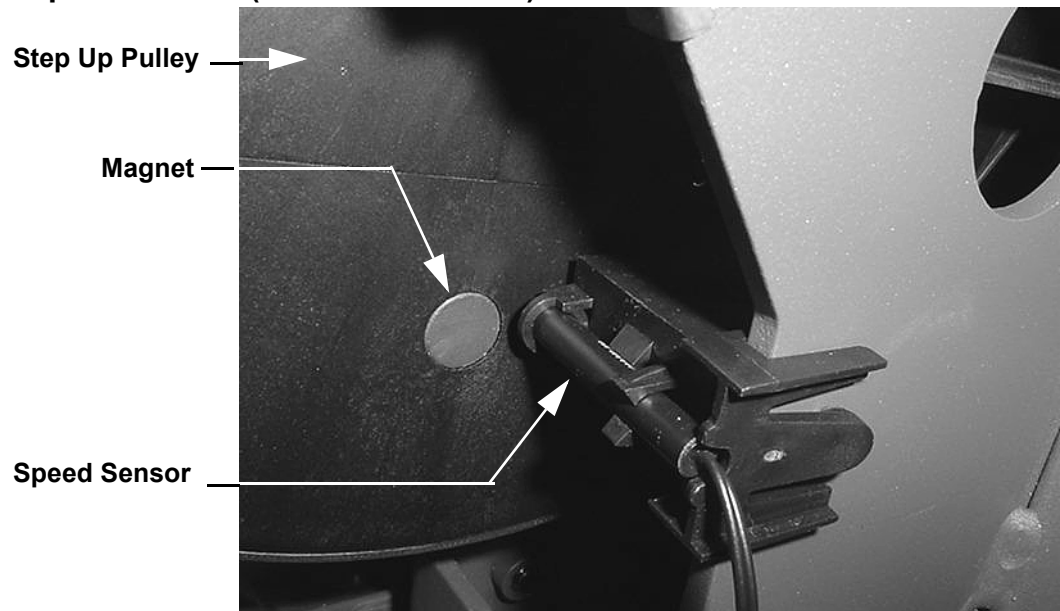
Diagram 6.4 - Speed Sensor (serial code AMPF)
