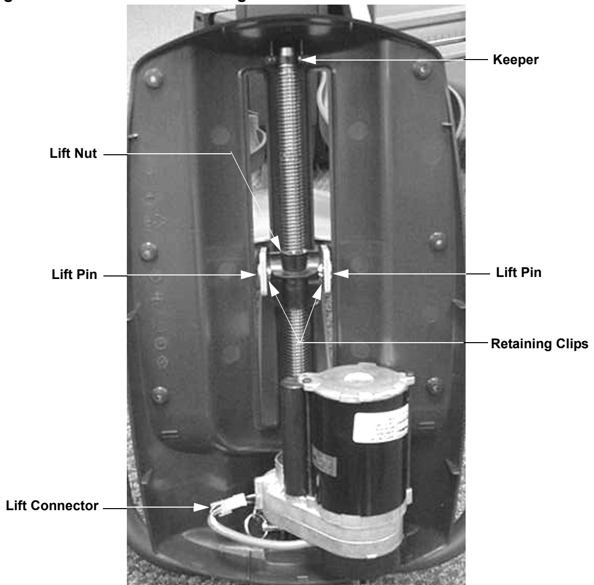
Diagram 7.25 - Lift Motor Mounting
