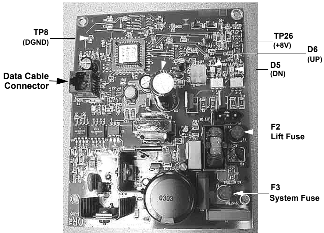
Diagram 6.5 - Lower PCA (Serial code SB)
