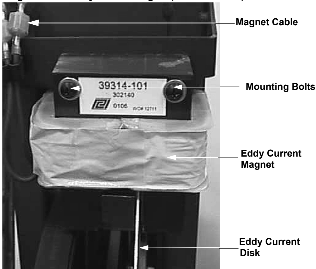
Diagram 7.15 - Eddy Current Magnet (Serial code SB)
