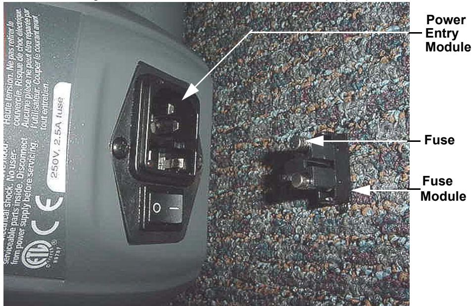
Diagram 7.24 - Power Entry Module Fuse (serial code AMPF)
